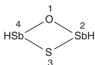
1,3,2,4-oxathiadistibetane
