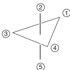
TBPY-5-25
