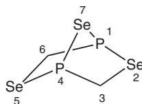
2,5,7-triseleno-1,4-diphosphabicyclo[2.2.1]heptane
