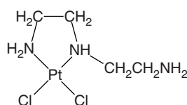
bidentate chelation
